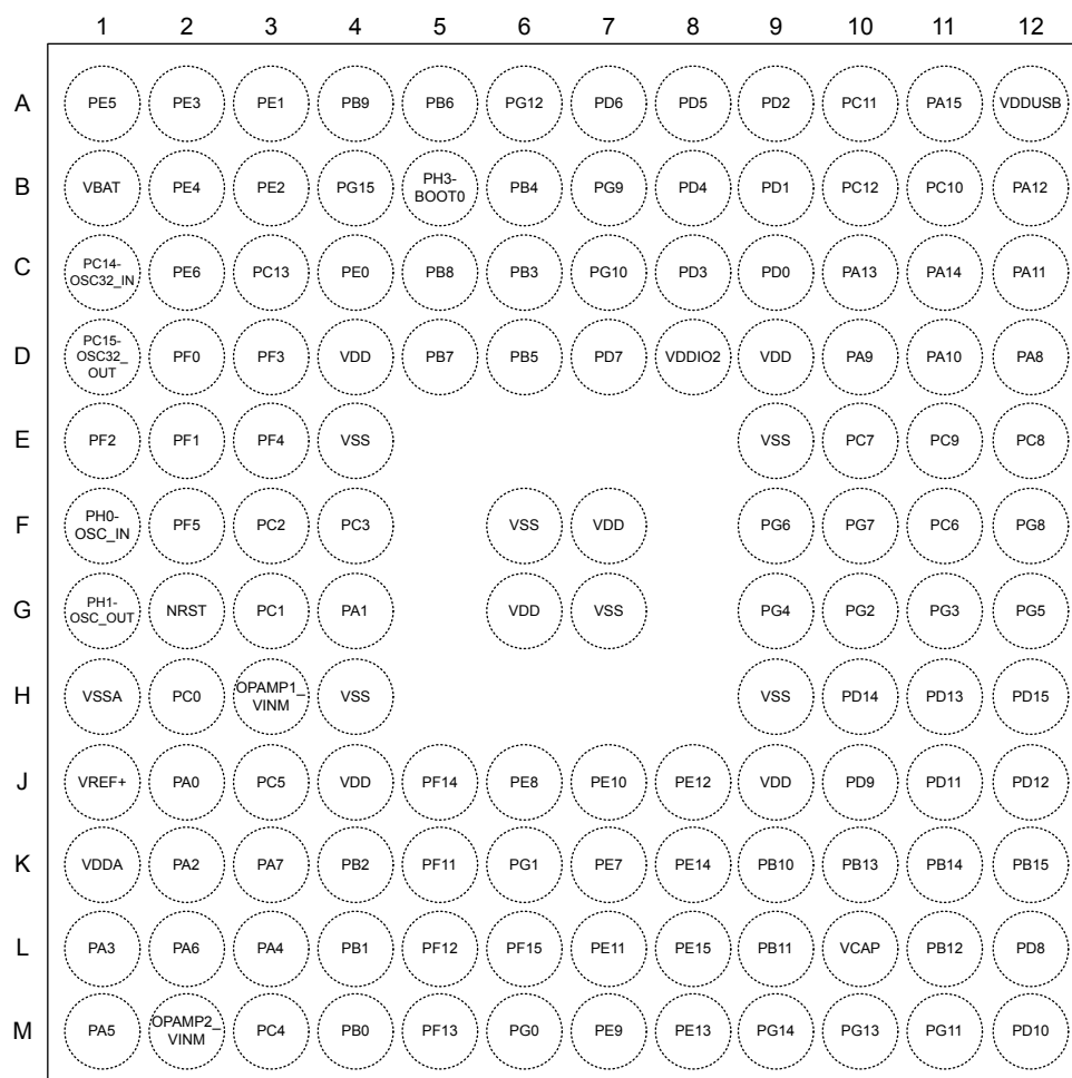
Figure 18. UFBGA132 ballout
