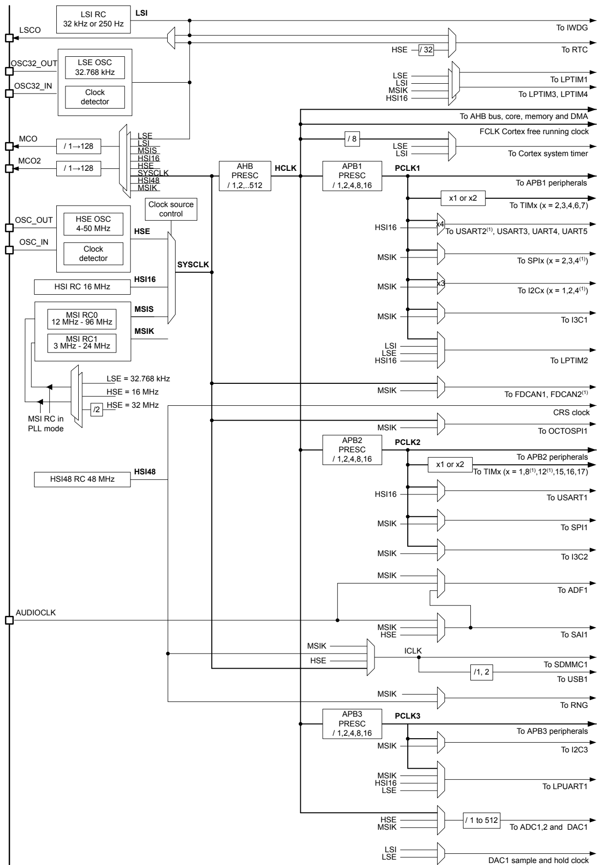
Figure 5. Clock tree
