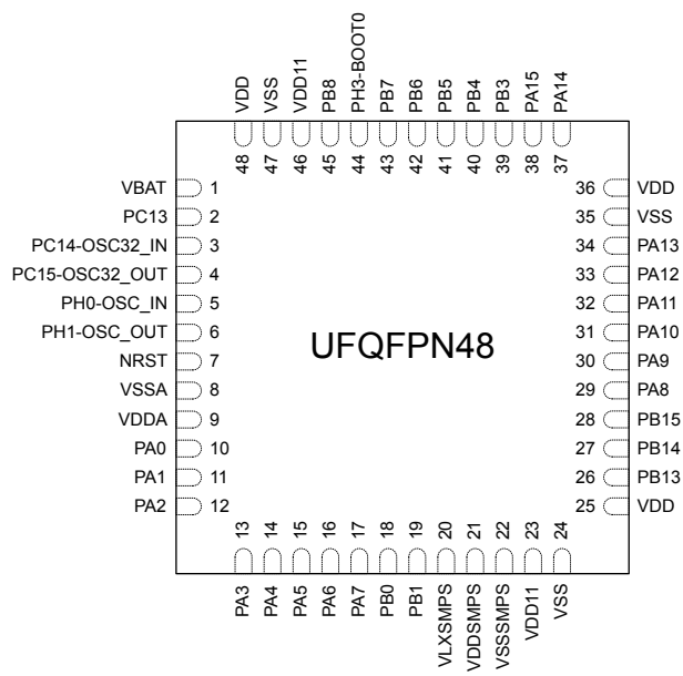
Figure 9. UFQFPN48 pinout
