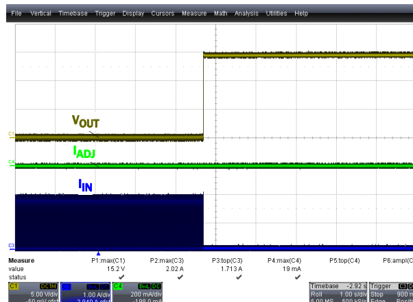
FIGURE 20. SHORT-CIRCUIT RECOVERY
