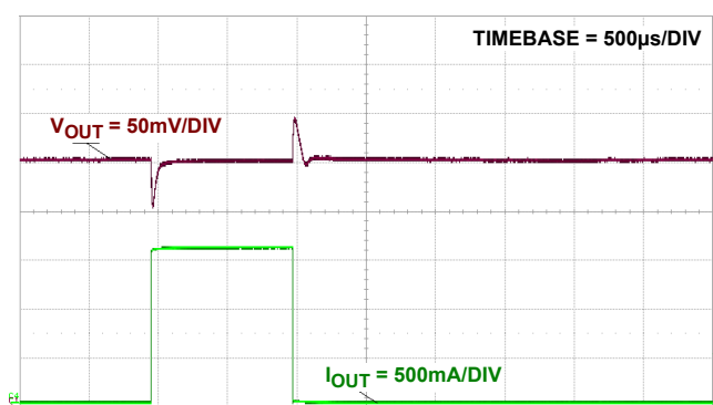
FIGURE 18. LOAD STEP RESPONSE, +25°C, V_{IN} = 13.2V , V_{OUT} = 10V , I_{OUT} = 0.15A TO 1.5A , C_{OUT} = 200\mu F , 30m\Omega
