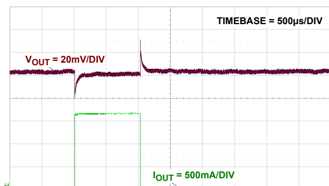
FIGURE 16. LOAD STEP RESPONSE, +25^{\circ}C , V_{IN} = 4.0V , V_{OUT} = 2.5V , I_{OUT} = 0.15A TO 1.6A , C_{OUT} = 200\mu F , 30m\Omega
