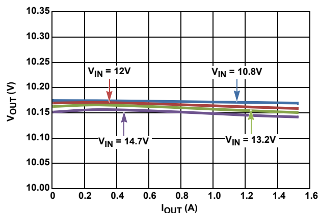
FIGURE 6. LOAD REGULATION V_{\text{OUT}} = 10.17\text{V} AT +25^{\circ}\text{C}
