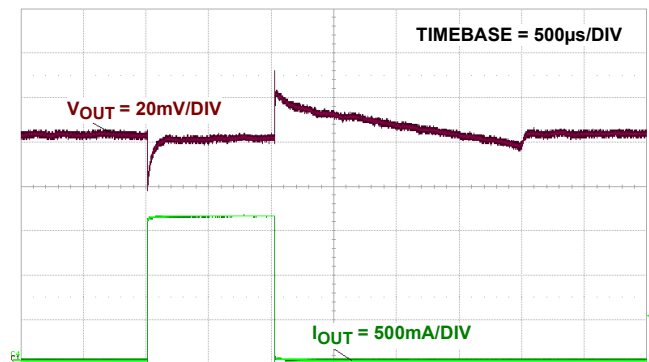
FIGURE 15. LOAD STEP RESPONSE +25^{\circ}C , V_{IN} = 4.0V , V_{OUT} = 2.5V , I_{OUT} = 0A TO 1.6A , C_{OUT} = 200\mu F , 30m\Omega
