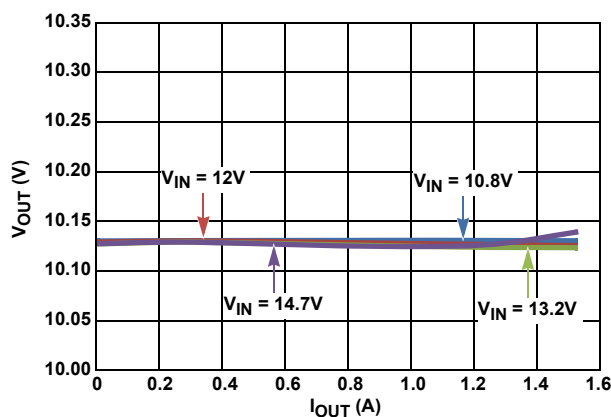
FIGURE 7. LOAD REGULATION V_{\text{OUT}} = 10.13\text{V} AT +125^{\circ}\text{C}
