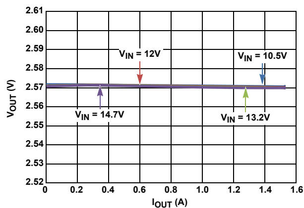
FIGURE 10. LOAD REGULATION V_{\text{OUT}} = 2.571\text{V} AT +125^{\circ}\text{C}
