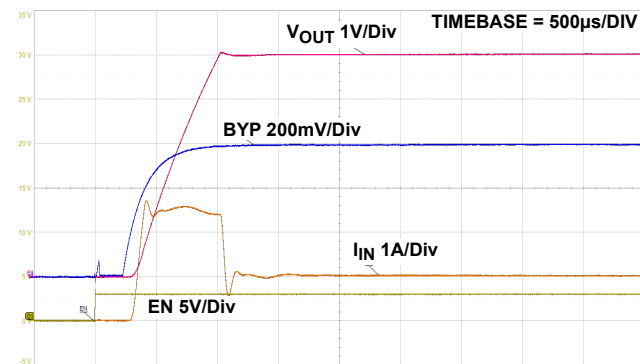
FIGURE 28. Soft-Start with BYP CAP = 0.2\mu F and EN to V_{OUT} Delay with VCCX CAP = 0.1\mu F , V_{IN} = 6.5V , V_{OUT} = 5V , R_L = 5\Omega , C_{OUT} = 220\mu F , ROCP = 300\Omega
