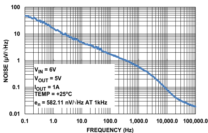
FIGURE 22. OUTPUT NOISE DENSITY
