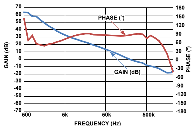
FIGURE 19. GAIN PHASE PLOTS, V_{IN} = 4V , V_{OUT} = 2.5V , I_{OUT} = 1.5A , R_{COMP} = 22k , C_{COMP} = 1nF , C_{OUT} = 200\mu F , 30m\Omega , PHASE MARGIN = 98.68°, GAIN MARGIN = 23.01dB
