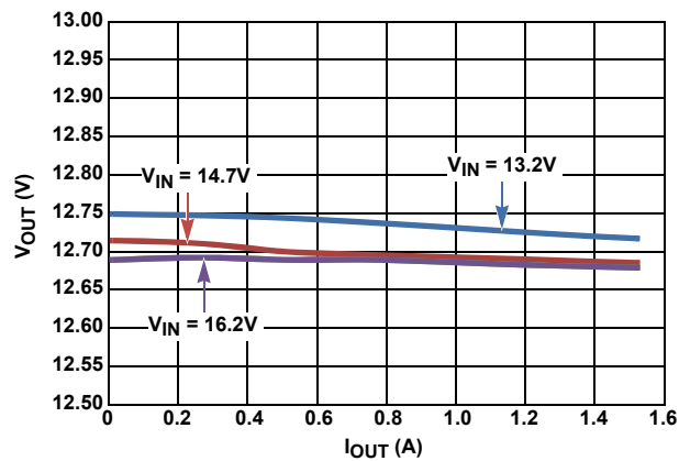
FIGURE 12. LOAD REGULATION V_{OUT} = 12.75V AT +25^{\circ}C
