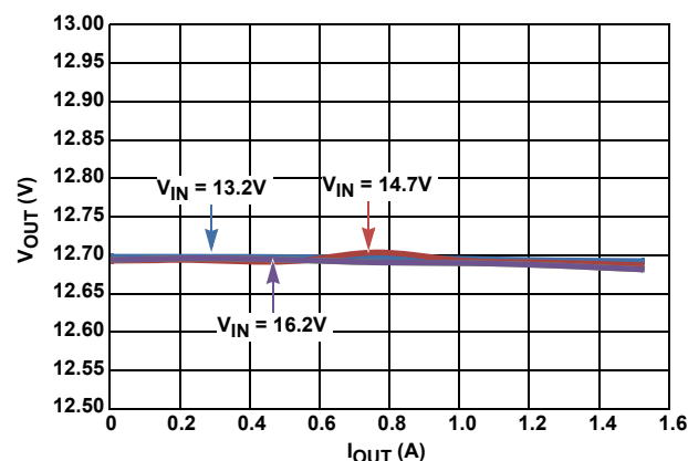
FIGURE 14. LOAD REGULATION V_{OUT} = 12.7V AT -55^{\circ}C
