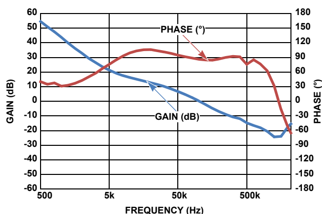
FIGURE 20. GAIN PHASE PLOTS, V_{IN} = 11V , V_{OUT} = 10V , I_{OUT} = 1.5A , R_{COMP} = 22k , C_{COMP} = 1nF , C_{OUT} = 200\mu F , 30m\Omega , PHASE MARGIN = 84.56°, GAIN MARGIN = 18.06dB
