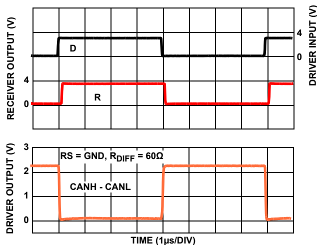
FIGURE 40. FAST DRIVER AND RECEIVER WAVEFORMS
