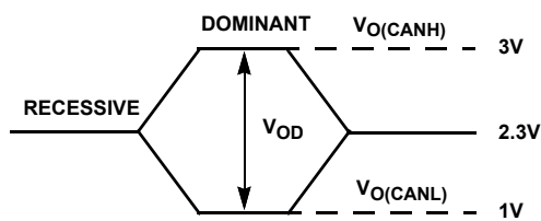
FIGURE 11. DRIVER BUS VOLTAGE DEFINITIONS
