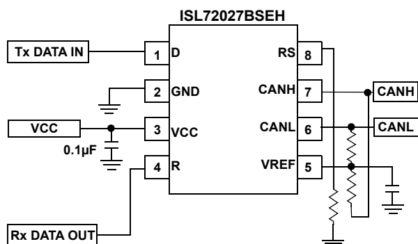
FIGURE 1. TYPICAL APPLICATION
