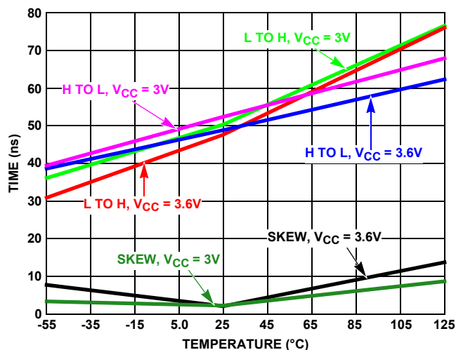
FIGURE 37. RECEIVER PROPAGATION DELAY AND SKEW vs TEMPERATURE
