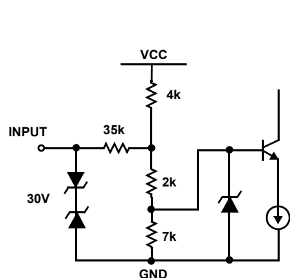
FIGURE 3. CANH AND CANL INPUTS
