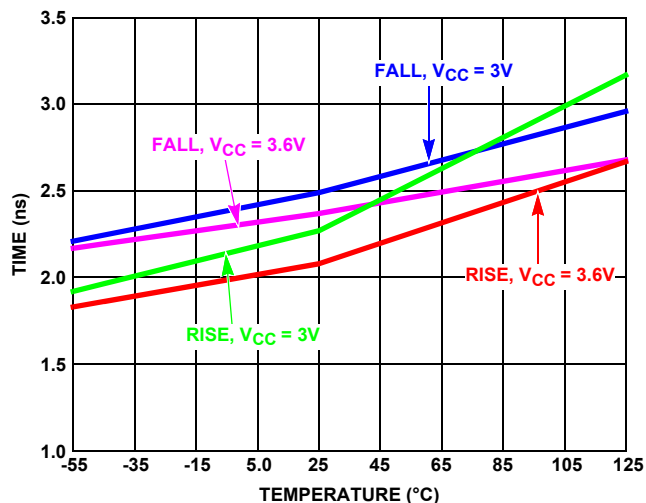
FIGURE 38. RECEIVER RISE AND FALL TIMES vs TEMPERATURE
