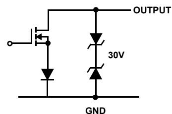
FIGURE 5. CANL OUTPUT
