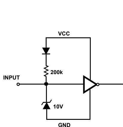
FIGURE 6. D INPUT
