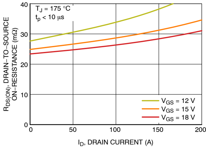
Figure 7. R_{DS(ON)} vs. I_D
