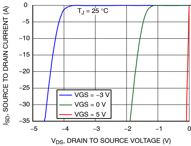
Figure 7. Reverse Conduction Characteristics at T_J = 25^\circ\text{C}
