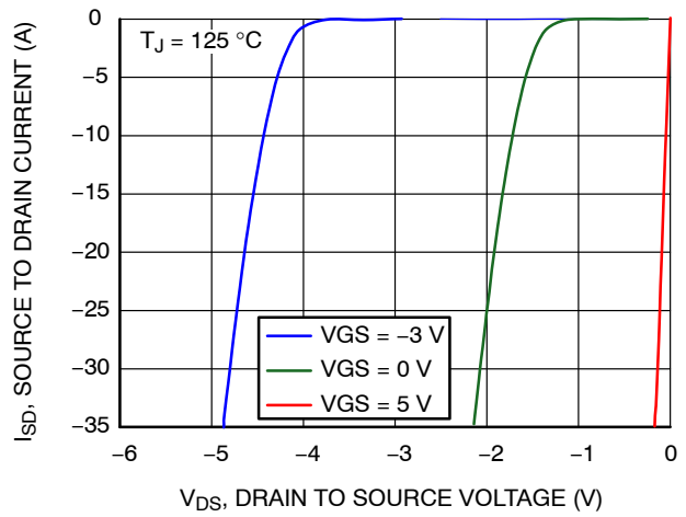
Figure 8. Reverse Conduction Characteristics at T_J = 125^\circ\text{C}
