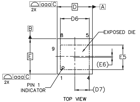
PTFP-N9 3.30x3.30x0.87, 0.65P CASE 522AE ISSUE O
