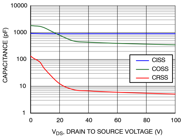
Figure 11. Capacitance Characteristics
