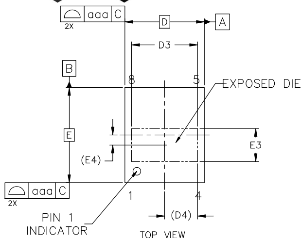
PDSO-N8 5.00x6.00x0.87, 1.27P CASE 144AD ISSUE A
