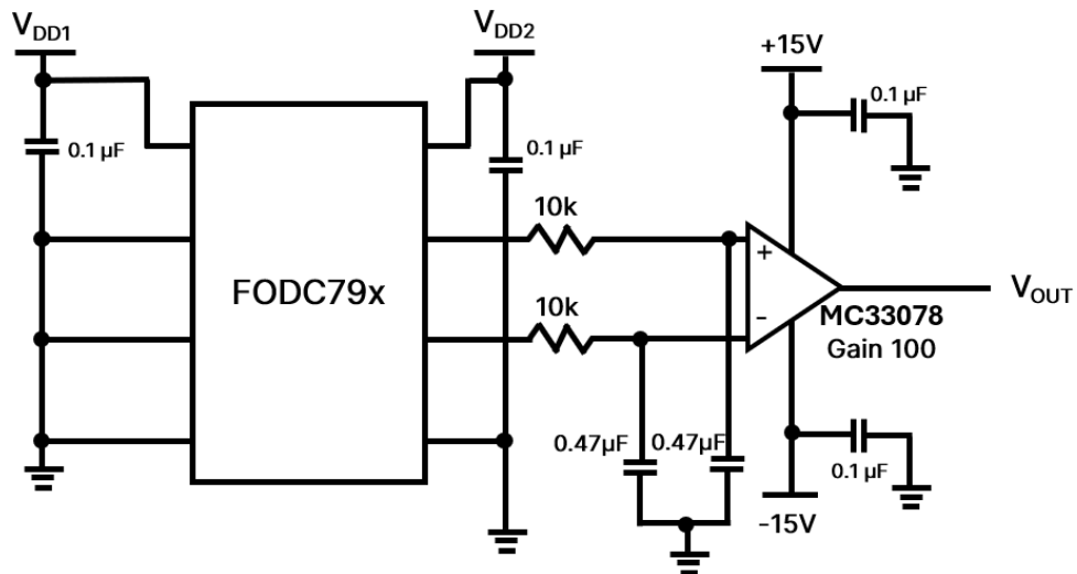
Figure 2. Input Voltage Test Circuit
