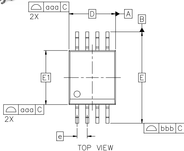
SOIC/LSOP-8 5.84x6.80x3.18, 1.27P CASE 751FC ISSUE O
