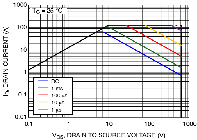
Figure 15. Safe Operating Area at T_C = 25^\circ\text{C}
