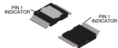
PDSO-G16 9.90 x 10.15 x 2.30, 1.20P CASE 208AA
