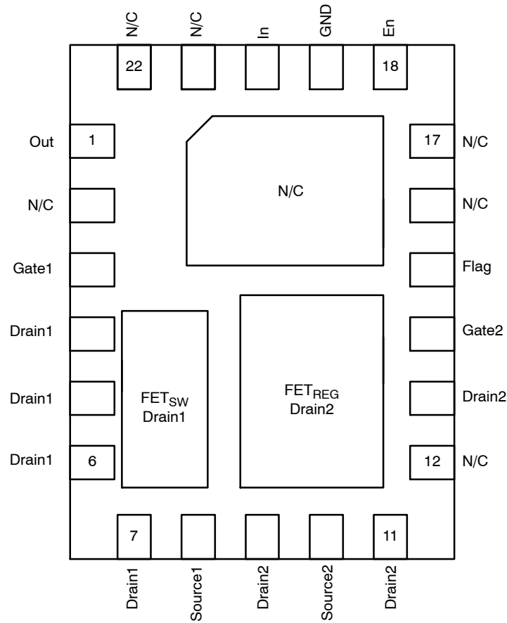
Figure 1. Pinout
