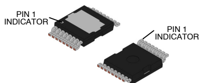
PDSO-G16 9.90x10.15x2.30, 1.20P CASE 208AA ISSUE A
