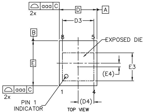
PDSO-N8 5.00x6.00x0.87, 1.27P CASE 144AE ISSUE O
