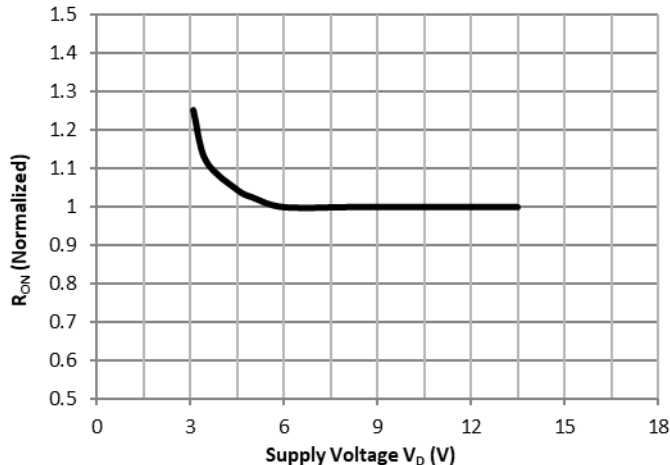
Figure 10. ON-state Resistance
