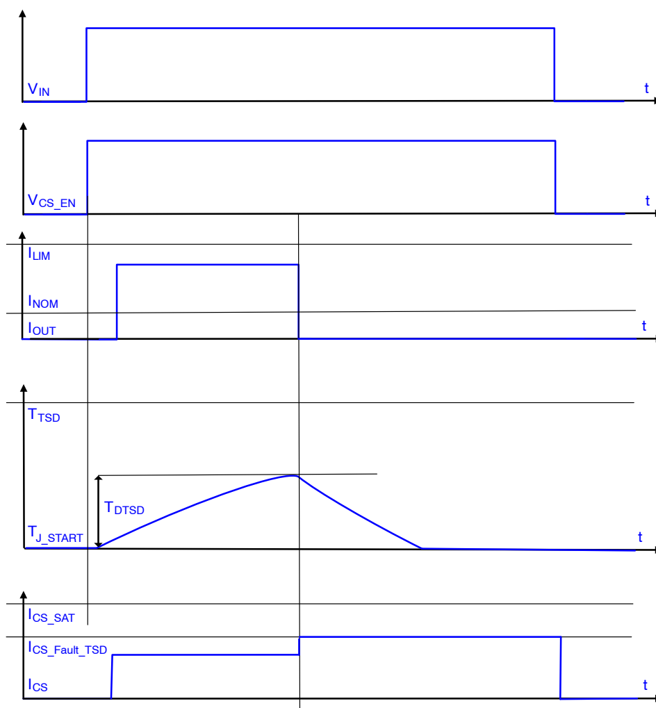
Figure 17. Over-Temperature Protection
