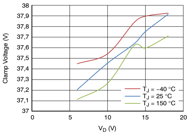
Figure 32. Drain-to-Source Clamping vs. T_J
