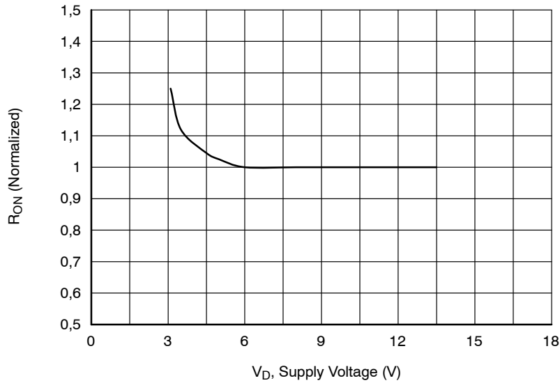
Figure 6. ON-state Resistance
