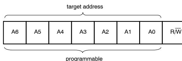
Figure 5. NLA9555 device Address
