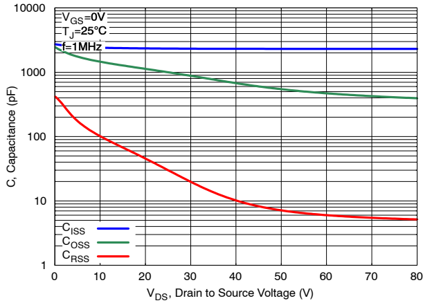
Figure 7. Capacitance Characteristics
