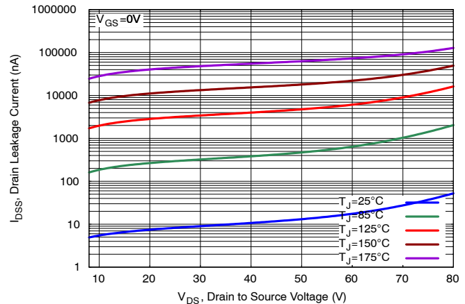
Figure 6. Drain Leakage Current vs. Drain Voltage
