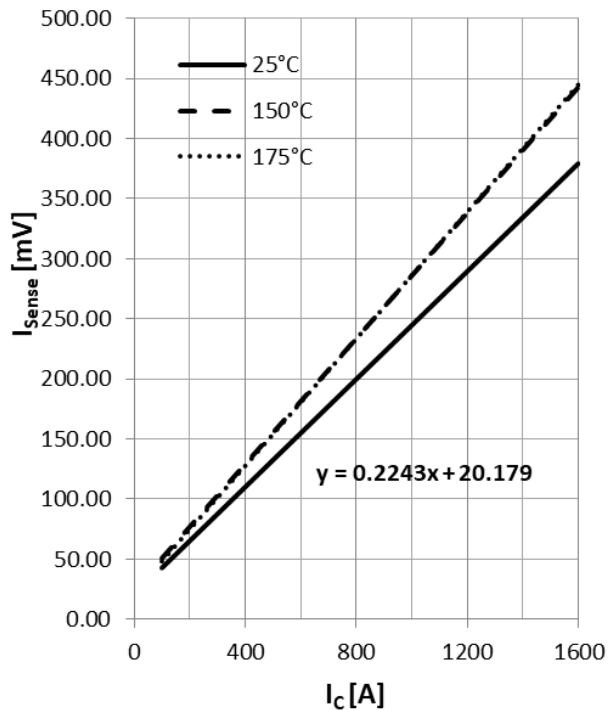
Figure 20. Current Sensor Characteristic
