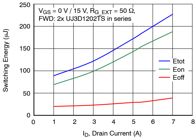
Figure 19. Clamped Inductive Switching Energy vs. Drain Current at V_{\text{DS}} = 1200 \text{ V} and T_J = 25^\circ\text{C}
