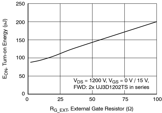
Figure 21. Clamped Inductive Switching Turn-on Energy vs. Gate Resistor R_{\text{G\_EXT}}
