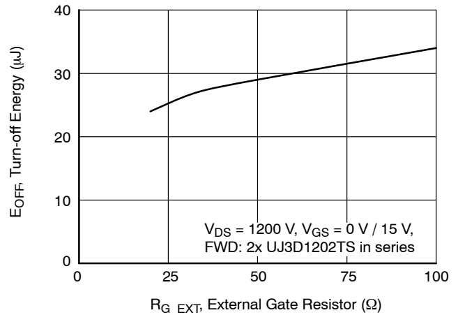
Figure 22. Clamped Inductive Switching Turn-off Energy vs. Gate Resistor R_{\text{G\_EXT}}
