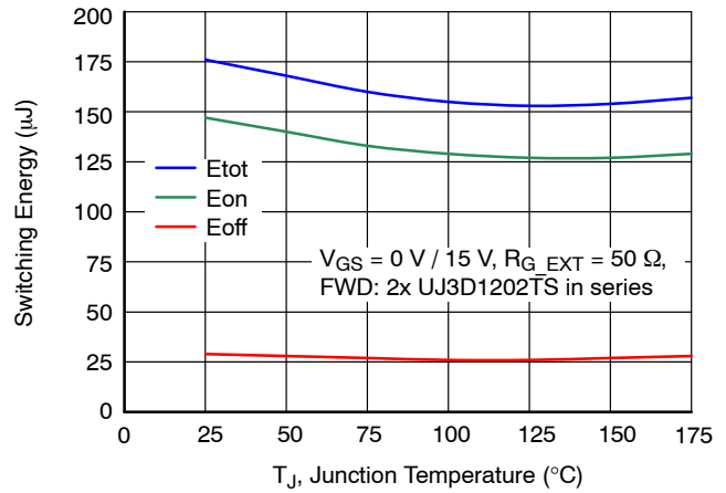
Figure 20. Clamped Inductive Switching Energy vs. Junction Temperature at V_{\text{DS}} = 1200 \text{ V} , and I_D = 5 \text{ A}
