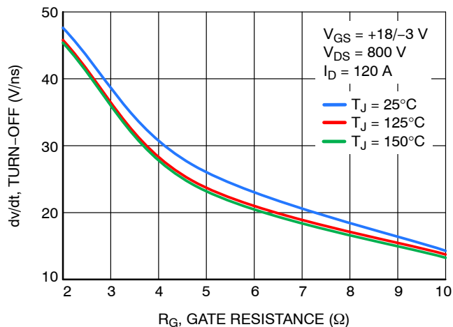
Figure 24. dv/dt Turn OFF vs. Gate Resistance V_{DS} = 800\text{ V}
