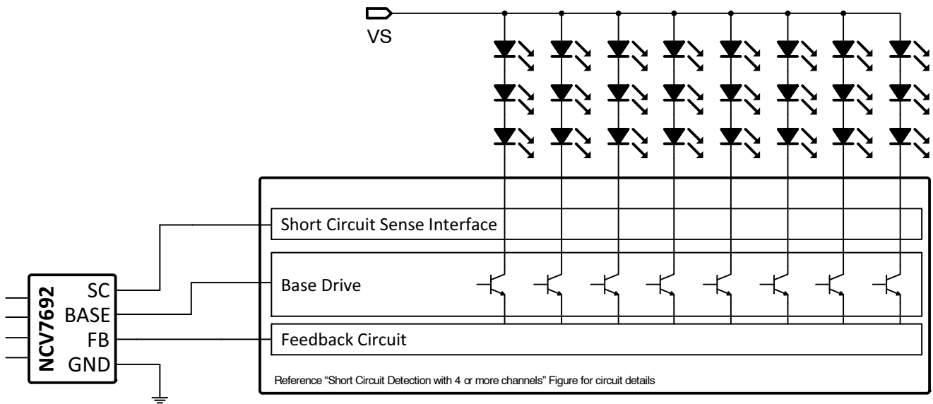
Figure 1. Application Diagram
