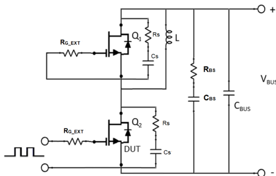
Figure 35. Schematic of the Half-Bridge Mode Switching Test Circuit. Note, a Bus RC Snubber ( R_{BS} = 5\Omega , C_{BS} = 100 nF) is Used to Reduce the Power Loop High Frequency Oscillations.
