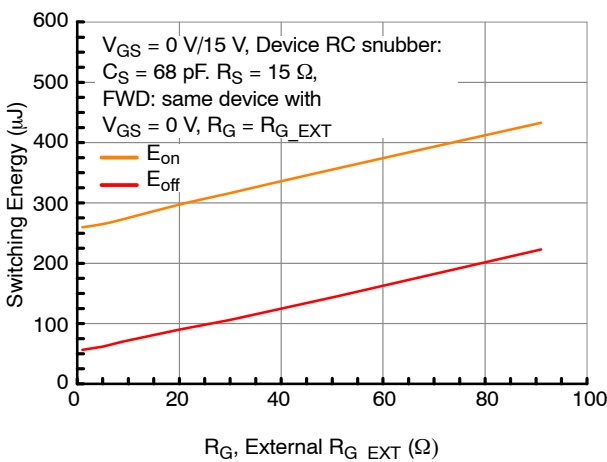
Figure 23. Clamped Inductive Switching Energies vs. R_{G\_EXT} at V_{DS} = 400 V, I_D = 25 A and T_J = 25 °C
