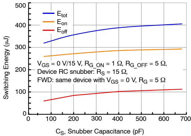
Figure 25. Clamped Inductive Switching Energies vs. Snubber Capacitance C_S at V_{DS} = 400 \text{ V} , I_D = 25 \text{ A} and T_J = 25 \text{ } ^\circ\text{C}
