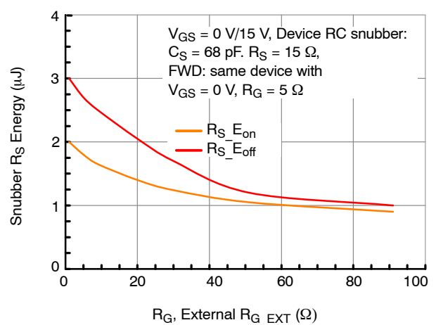
Figure 24. RC Snubber Energy Losses vs. R_{G\_EXT} at V_{DS} = 400 V, I_D = 25 A and T_J = 25 °C
