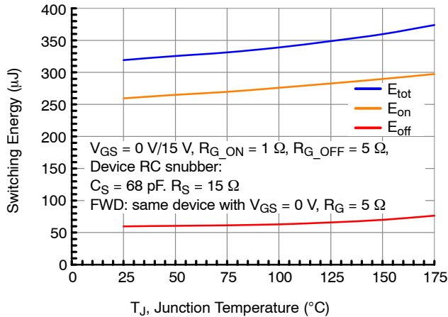
Figure 27. Clamped Inductive Switching Energy vs. Junction Temperature at V_{DS} = 400 \text{ V} and I_D = 25 \text{ A}
