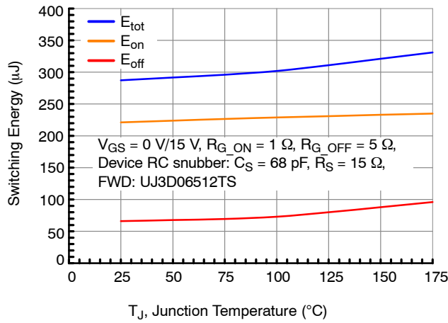
Figure 33. Clamped Inductive Switching Energy vs. Junction Temperature at V_{DS} = 400 V and I_D = 25 A
