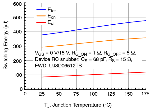
Figure 34. Clamped Inductive Switching Energy vs. Junction Temperature at V_{DS} = 500 V and I_D = 25 A
