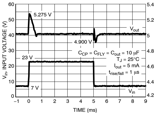
Figure 14. Line Transient
