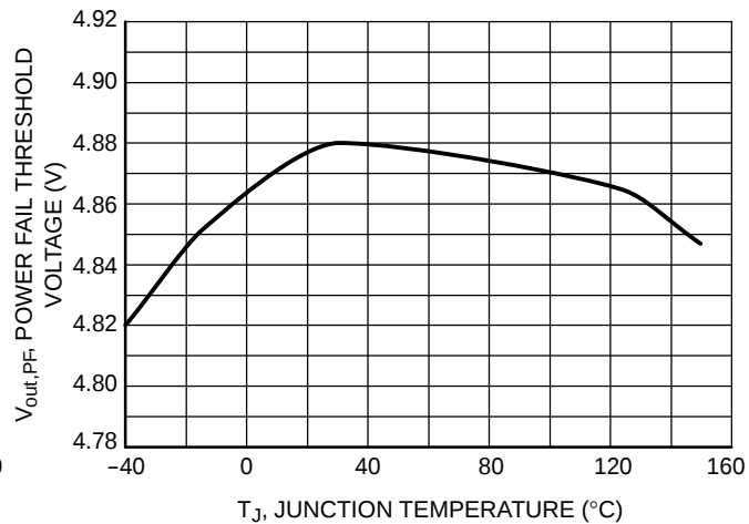
Figure 11. Power Fail Threshold Voltage vs. Junction Temperature
