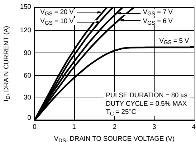
Figure 8. Saturation Characteristics
