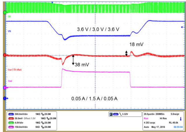
Figure 37. Transient load 0.05 to 1.5 A Transient line 3.6 – 3.0 V Forced PPW
