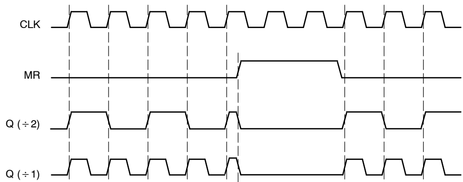
Figure 3. Master Reset (MR) Timing Diagram
