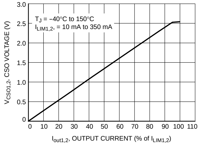
Figure 9. Output Current (% of I_{LIM} ) vs. CSO Voltage
