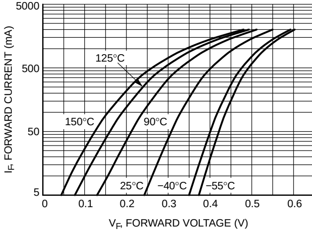
Figure 5. Forward Voltage
