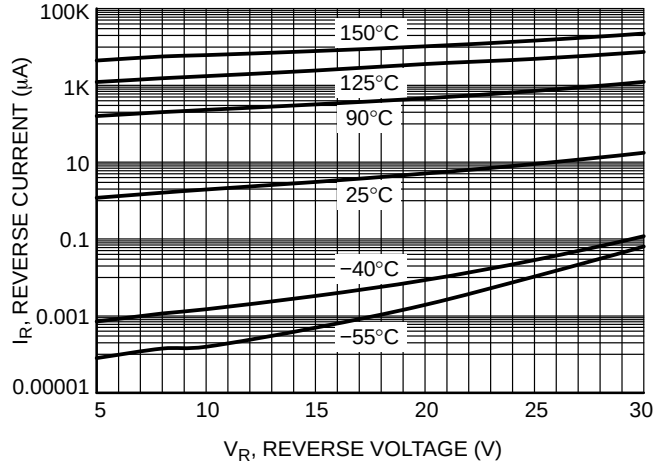
Figure 6. Leakage Current
