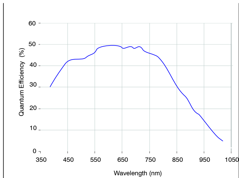
Figure 44. Typical Quantum Efficiency – Monochrome
