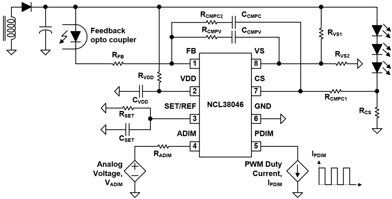
Figure 1. Application Schematic
