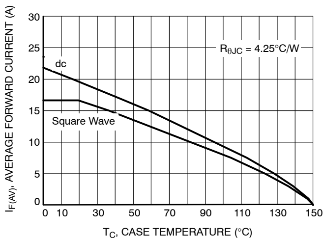
Figure 5. Current Derating TO-220 FULLPAK
