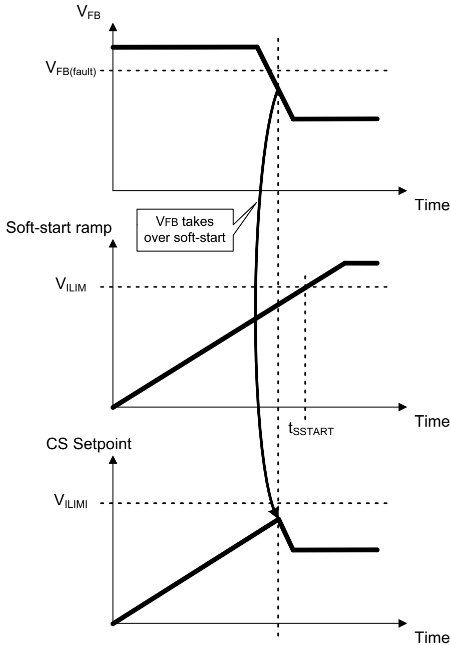
Figure 36. Soft-Start
