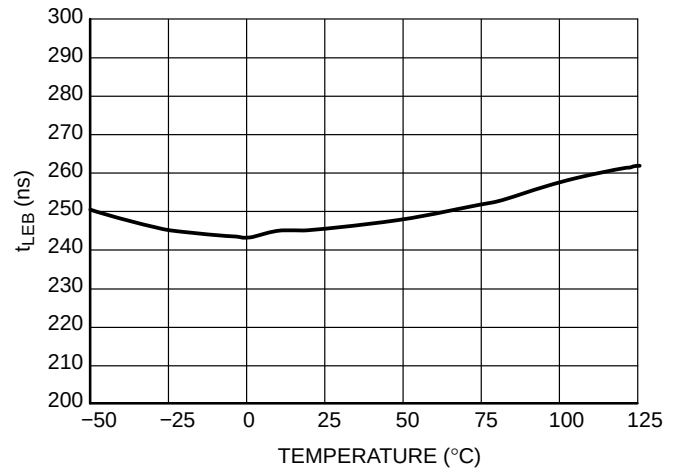
Figure 10. Leading Edge Blanking Duration t_{\text{LEB}}
