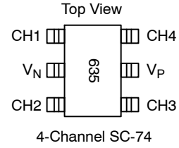
PACKAGE/PINOUT DIAGRAM
