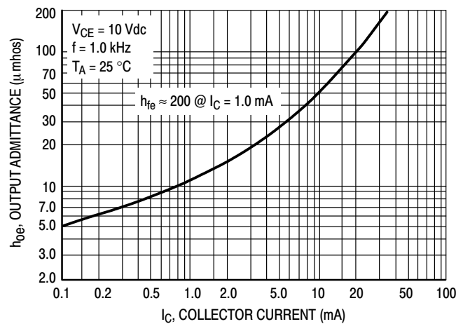
Figure 19. Output Admittance
