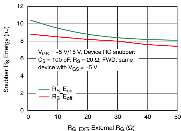
Figure 22. RC Snubber Energy Loss vs. R_{G\_EXT} at V_{DS} = 800 \text{ V} , I_D = 20 \text{ A} , and T_J = 25^\circ \text{C}
