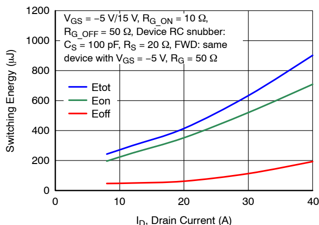
Figure 19. Clamped Inductive Switching Energy vs. Drain Current at V_{DS} = 800 \text{ V} and T_J = 25^\circ \text{C}
