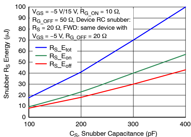
Figure 24. RC Snubber Energy Losses vs. Snubber Capacitance C_S at V_{DS} = 800 \text{ V} , I_D = 20 \text{ A} , and T_J = 25^\circ \text{C}
