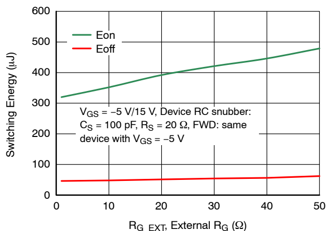
Figure 21. Clamped Inductive Switching Energies vs. R_{G\_EXT} at V_{DS} = 800 \text{ V} , I_D = 20 \text{ A} , and T_J = 25^\circ \text{C}
