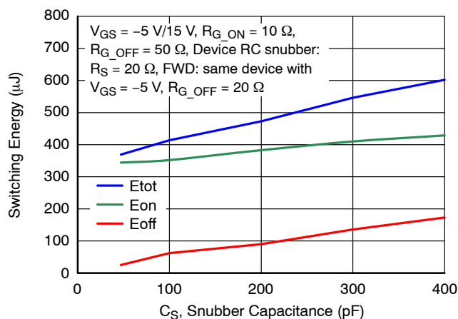
Figure 23. Clamped Inductive Switching Energies vs. Snubber Capacitance C_S at V_{DS} = 800 \text{ V} , I_D = 20 \text{ A} , and T_J = 25^\circ \text{C}
