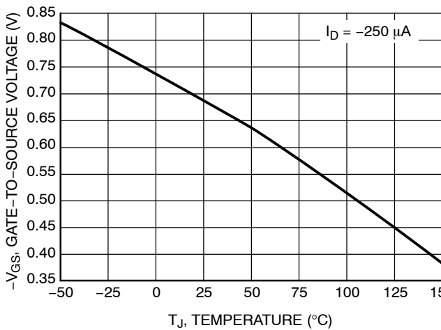
Figure 11. Threshold Voltage
