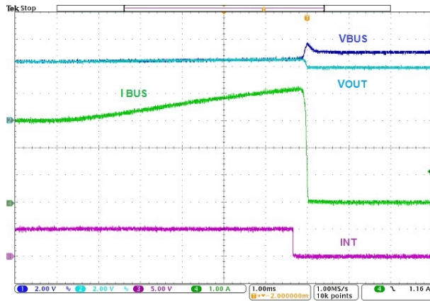
Figure 8. Switch Opening IBUS OCP Fault, [IBUSOCP]=4A , [IBUSREG]=[IBATREG]=\text{max} , T_A Current Limit Raised from 3 A to 5 A
