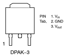
Figure 3. Pin Connections
