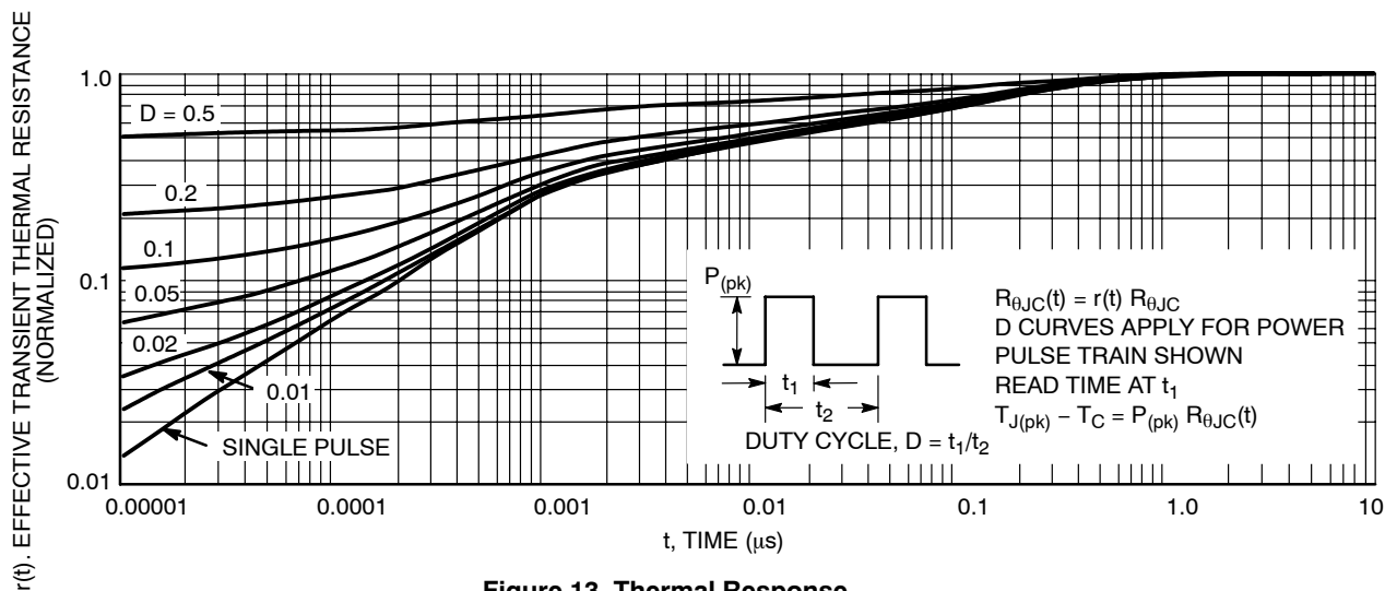
Figure 13. Thermal Response
