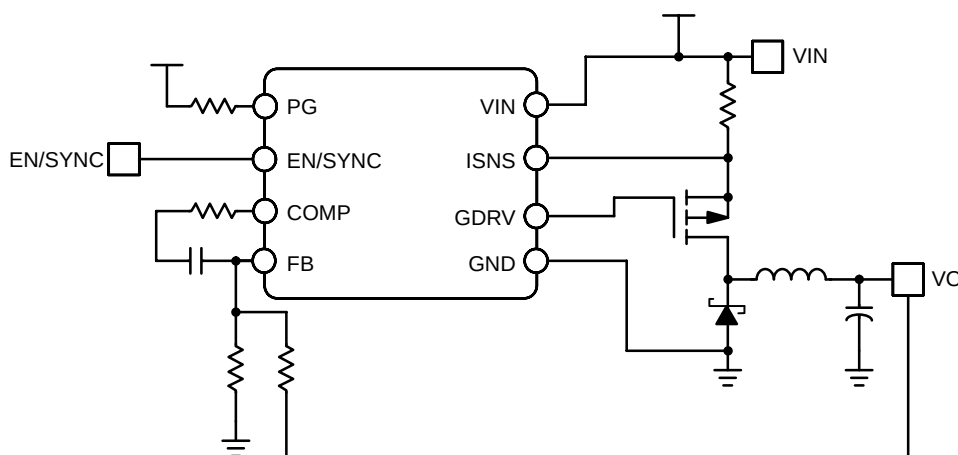
Figure 1. NCV8853 Application Diagram
