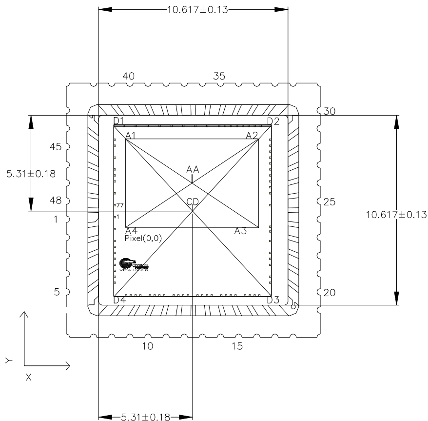
Figure 42. Graphical Representation of the Optical Center
