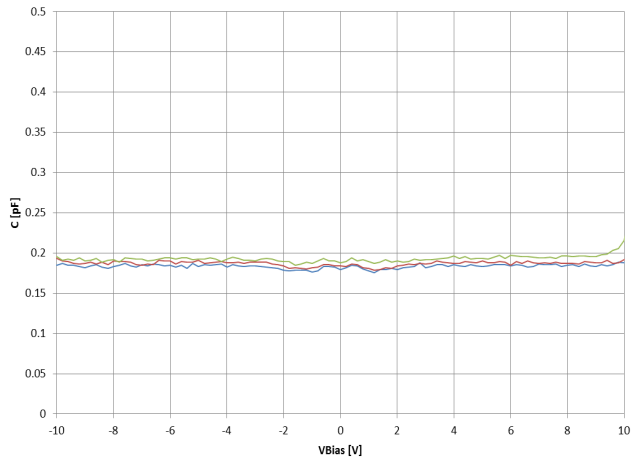
Figure 4. CV Characteristics
