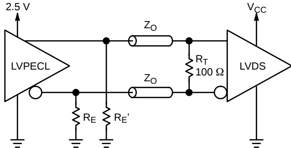
Figure 14. Interfacing 2.5 V LVPECL to LVDS with External 100 \Omega Termination Resistor
