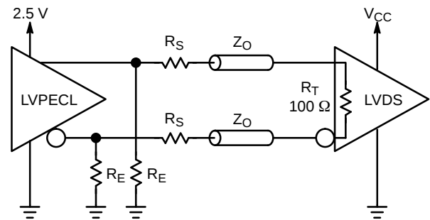
Figure 18. Interfacing 2.5 V LVPECL to LVDS with Series R_S and Internal 100 \Omega Termination Resistor
