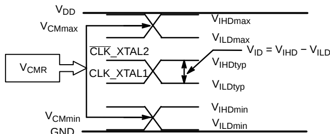
Figure 7. V_{CM} Diagram
