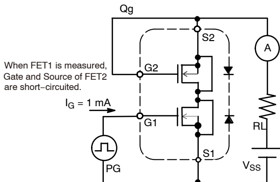
Figure 7. Test Circuit 7
