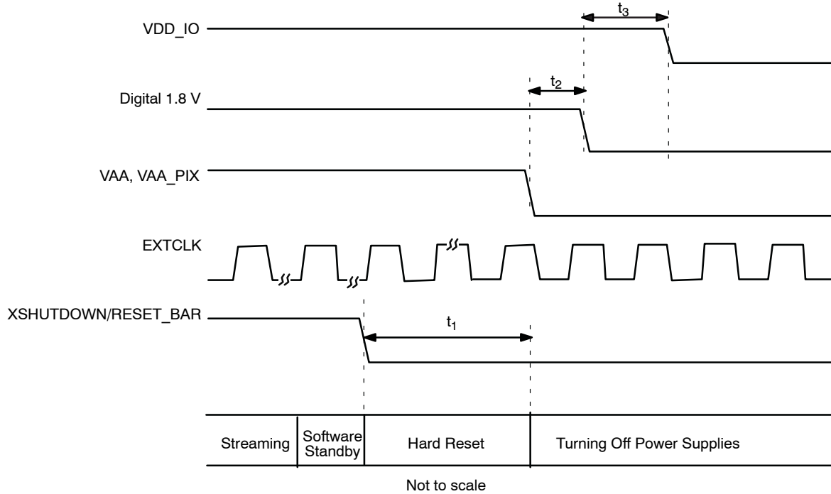
Figure 27. Power-Down Sequence
