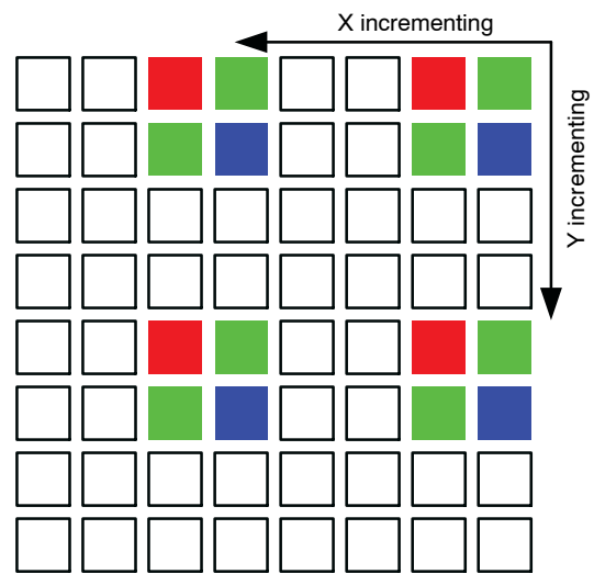
Figure 14. Pixel Readout ( x_{\text{odd\_inc}} = 3 , y_{\text{odd\_inc}} = 3 )
