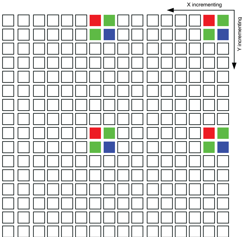
Figure 15. Pixel Readout ( x_{\text{odd\_inc}} = 7 , y_{\text{odd\_inc}} = 7 )
