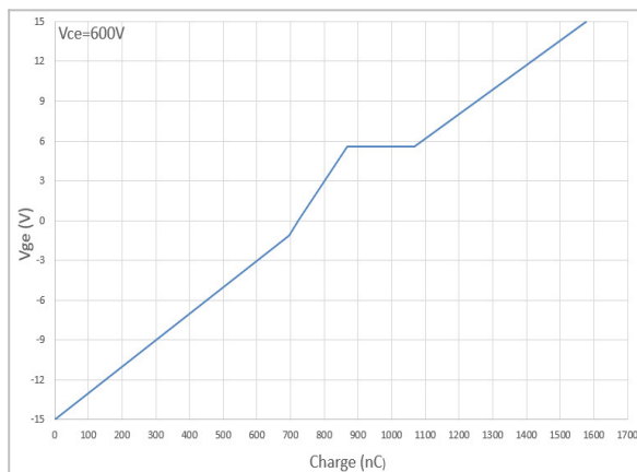
Figure 20. Gate Voltage vs. Gate Charge
