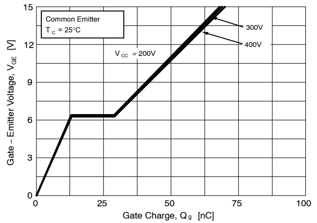
Figure 8. Gate Charge
