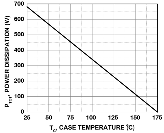
Figure 5. Power Derating
