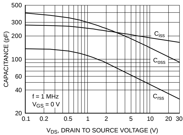
Figure 9. Capacitance Characteristics
