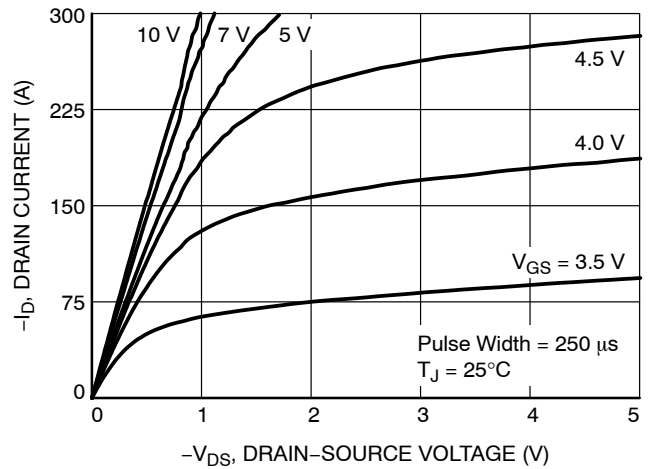
Figure 9. Saturation Characteristics
